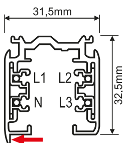
track cross-section. Bias line (marked in red)
